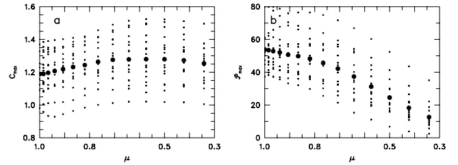
Fig. 7. Maximum contrast value a) and maximum polarization signal ( \mathcal{P} (Fe I 630.25)) b) as a function of disk position \mu .
