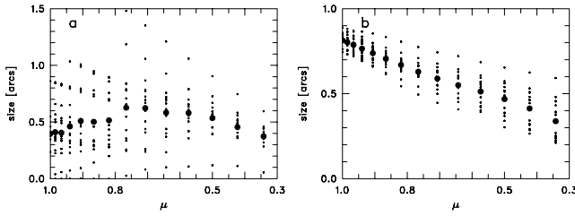
Fig. 6. Apparent size of contrast enhancement a) and polarization signal ( \mathcal{P} (Fe I 630.25)) b) as a function of disk position \mu . For each \mu < 1 there are 16 points from the 8 snapshots a)–h) of Fig. 5 and two opposite directions. The heavy dots show arithmetic means.
